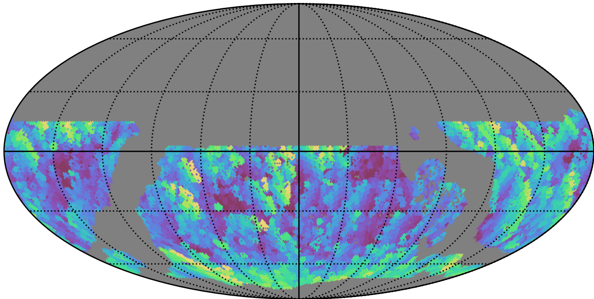
early_u_fpextra4.0_v3.4_10yrs WFD g band: Max airmass
