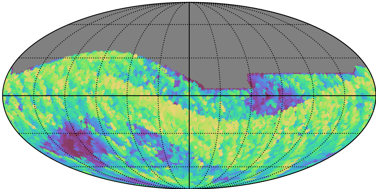
early_u_fpextra4.0_v3.4_10yrs All sky z band: Max airmass
