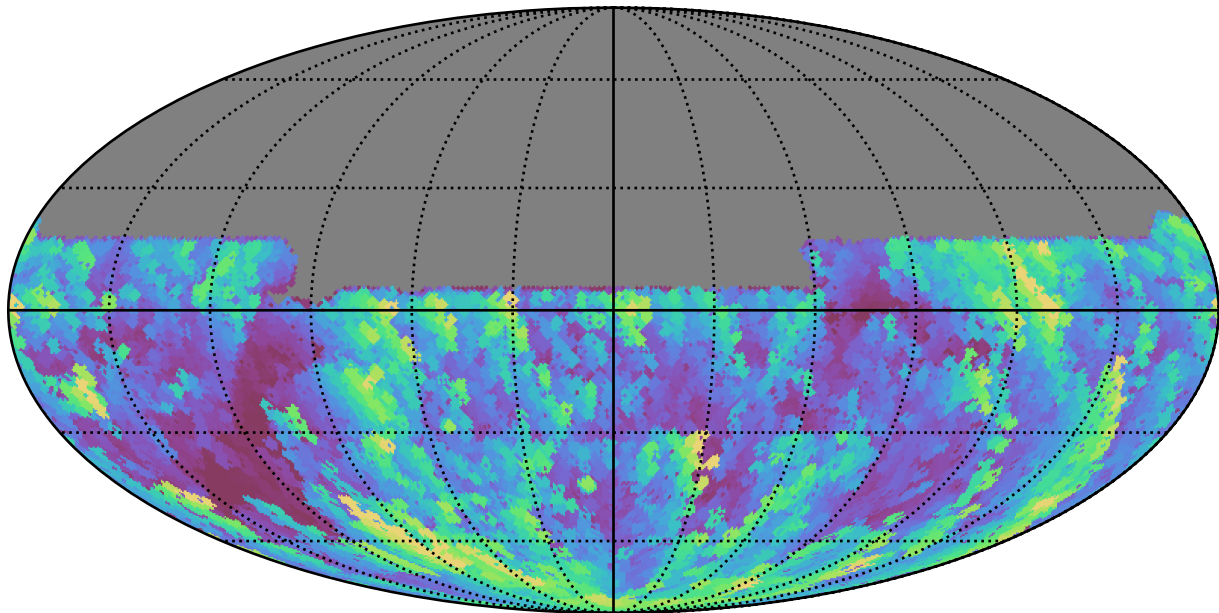
early_u_fpextra4.0_v3.4_10yrs All sky u band: Max airmass
