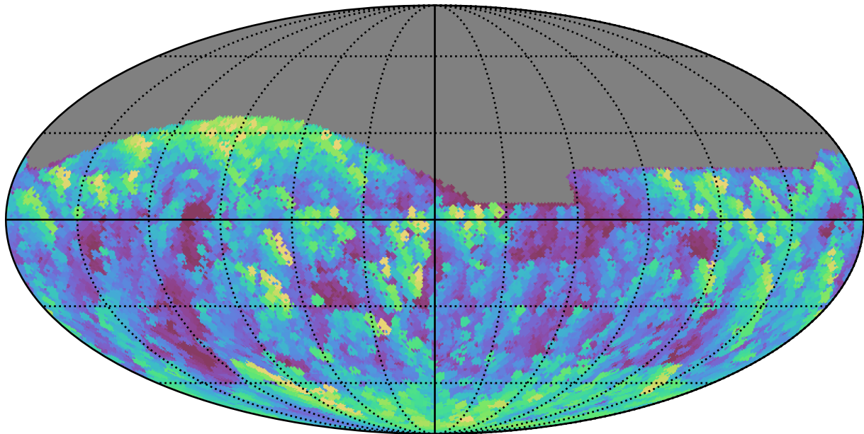
early_u_fpextra4.0_v3.4_10yrs All sky g band: Max airmass
