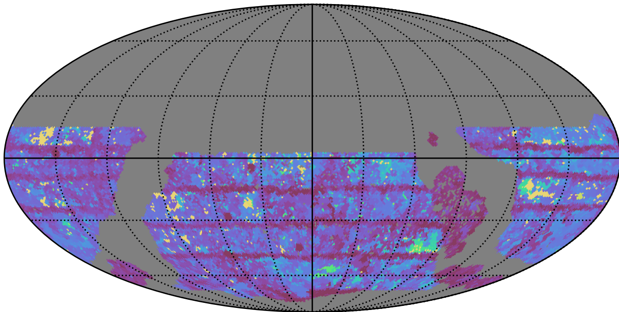
early_u_fpextra4.0_v3.4_10yrs WFD z band: Max Inter-Night Gap
