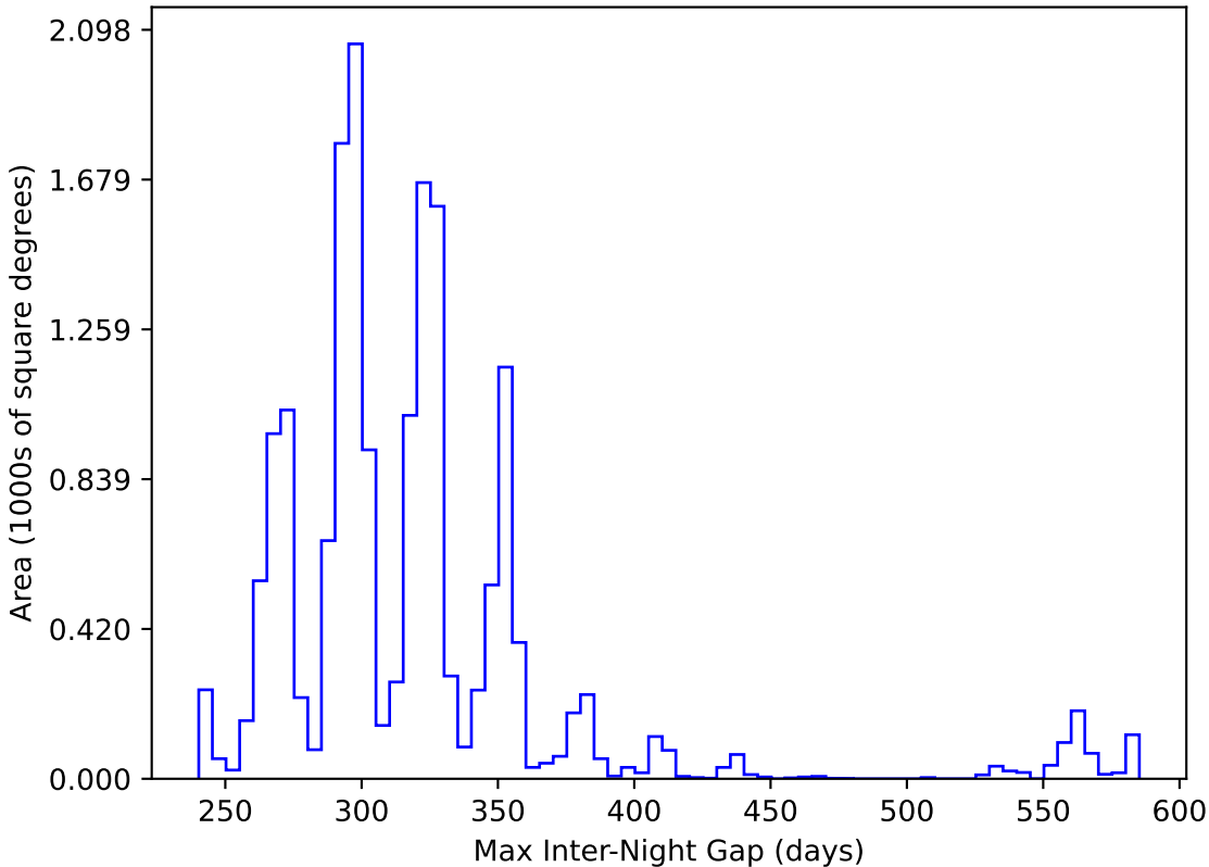
early_u_fpextra4.0_v3.4_10yrs WFD y band: Max Inter-Night Gap
