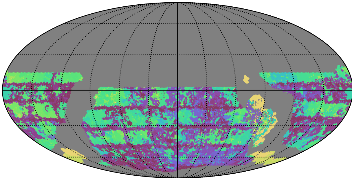
early_u_fpextra4.0_v3.4_10yrs WFD u band: Max Inter-Night Gap
