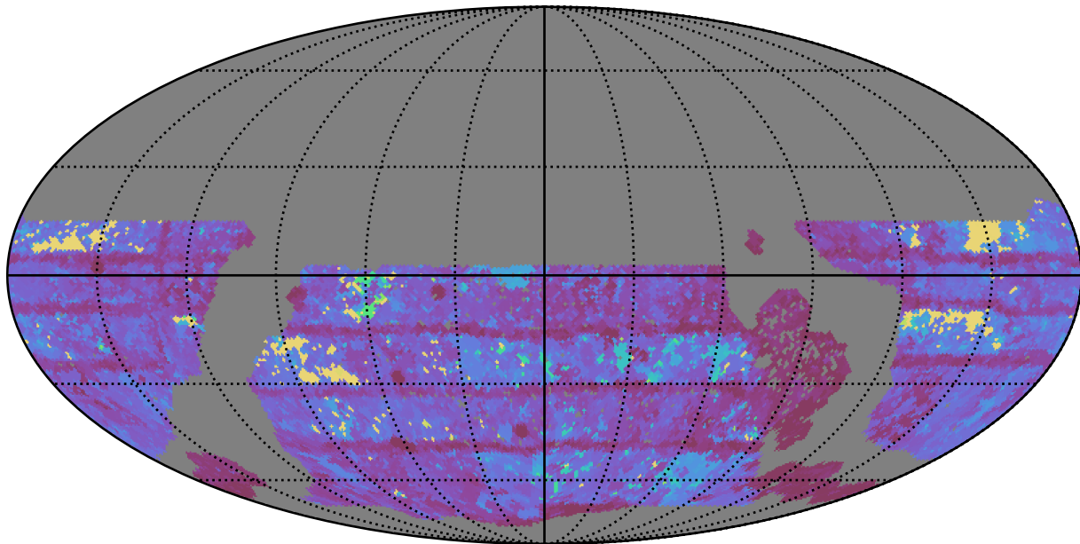
early_u_fpextra4.0_v3.4_10yrs WFD r band: Max Inter-Night Gap
