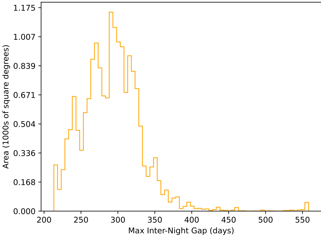
early_u_fpextra4.0_v3.4_10yrs WFD r band: Max Inter-Night Gap
