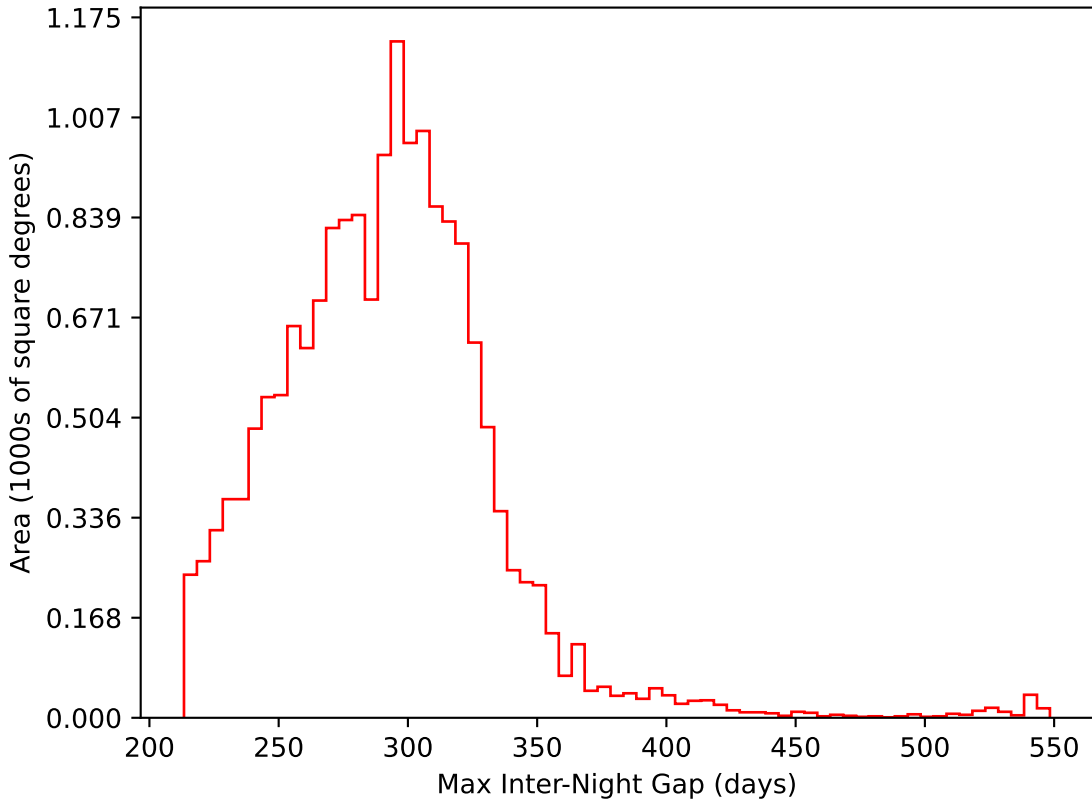
early_u_fpextra4.0_v3.4_10yrs WFD i band: Max Inter-Night Gap
