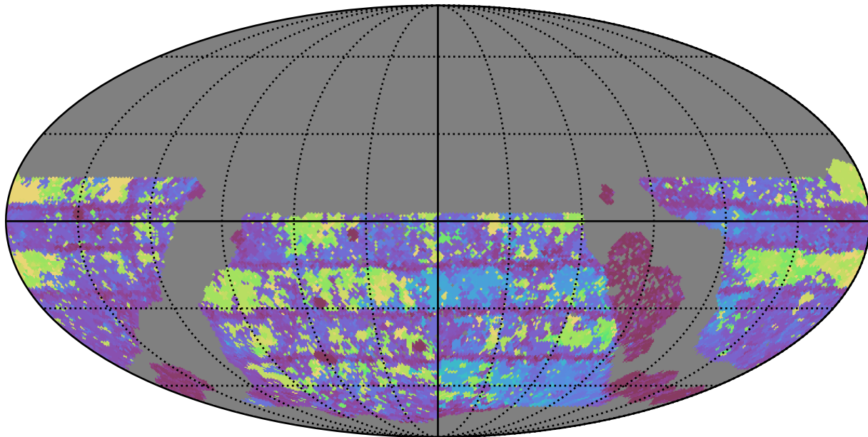
early_u_fpextra4.0_v3.4_10yrs WFD g band: Max Inter-Night Gap
