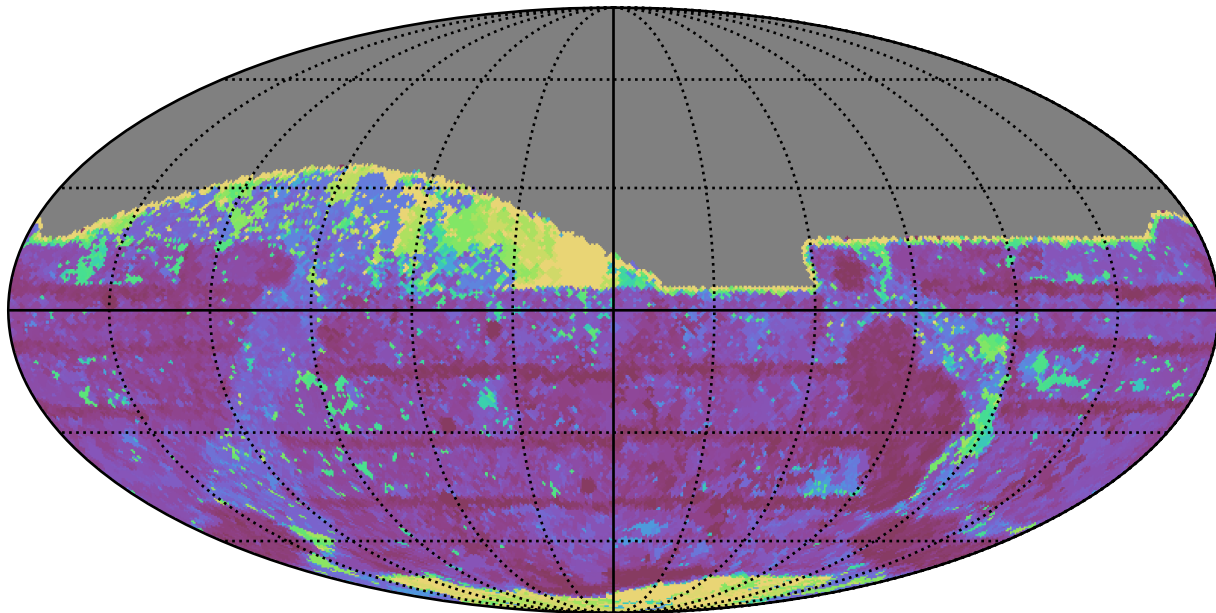
early_u_fpextra4.0_v3.4_10yrs All sky z band: Max Inter-Night Gap
