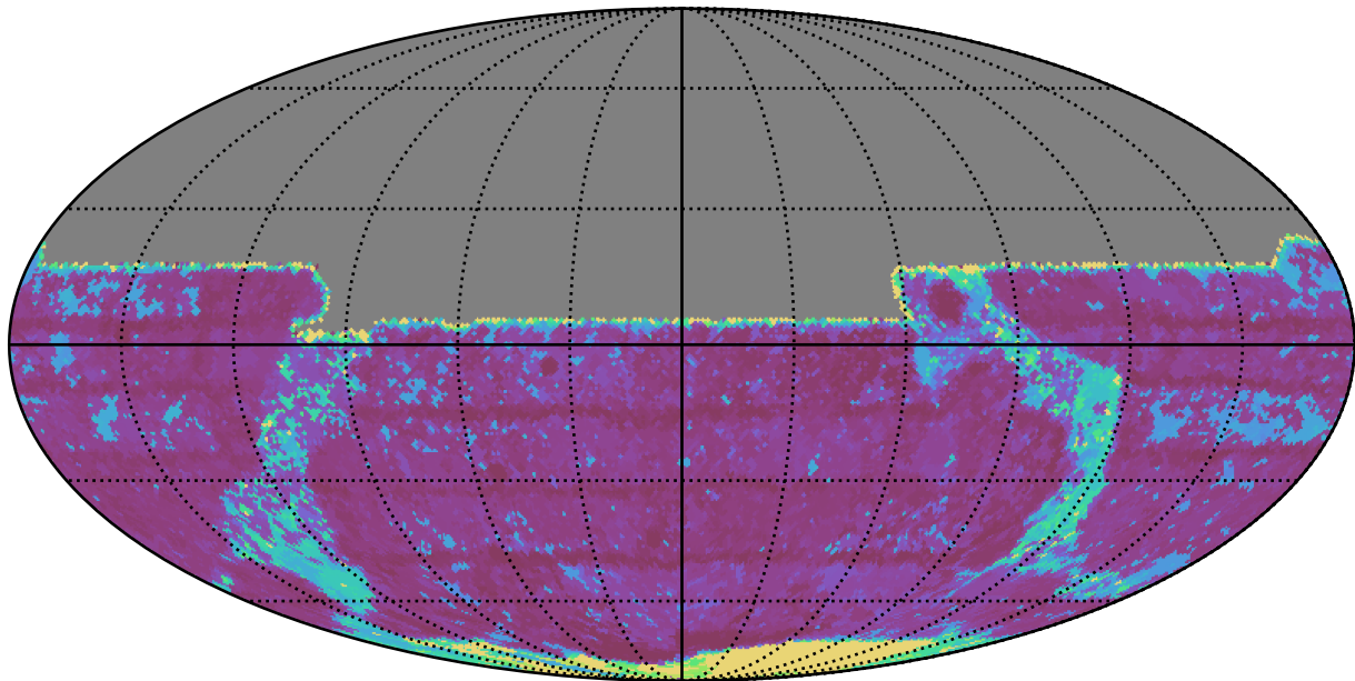
early_u_fpextra4.0_v3.4_10yrs All sky y band: Max Inter-Night Gap
