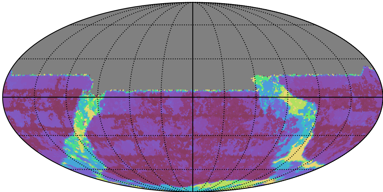
early_u_fpextra4.0_v3.4_10yrs All sky u band: Max Inter-Night Gap
