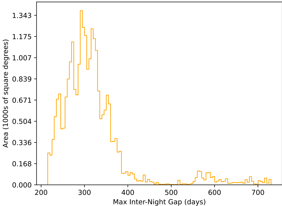
early_u_fpextra4.0_v3.4_10yrs All sky r band: Max Inter-Night Gap
