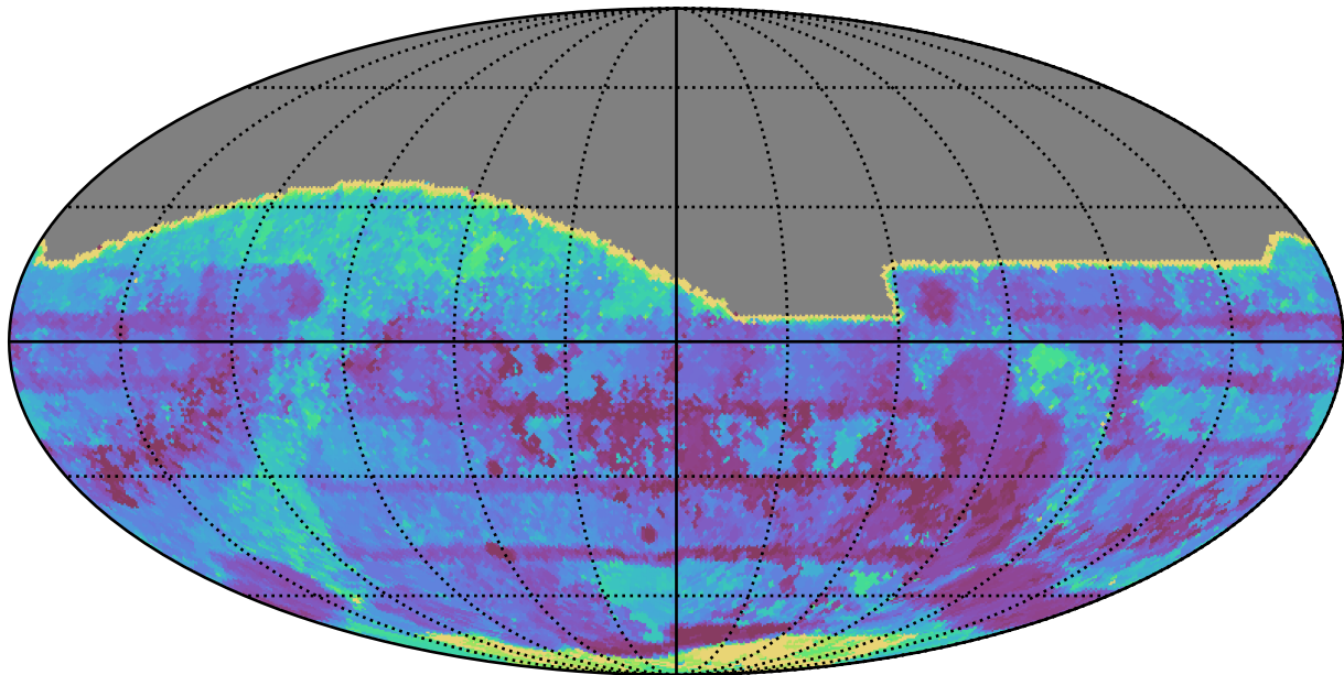
early_u_fpextra4.0_v3.4_10yrs All sky all bands: Max Inter-Night Gap
