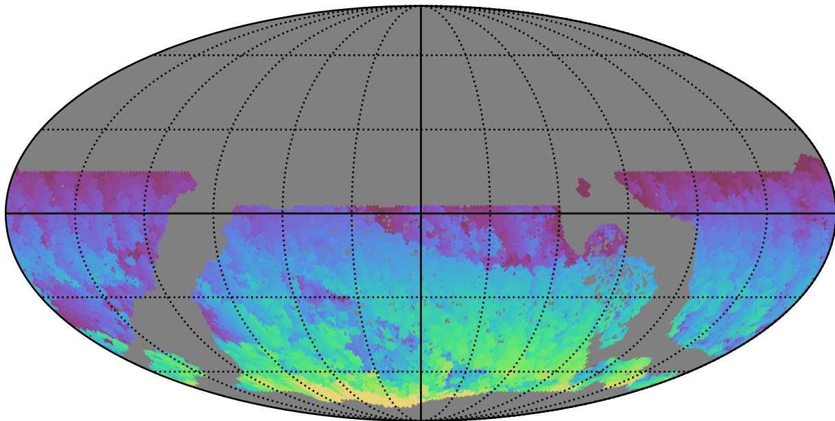
early_u_fpextra4.0_v3.4_10yrs WFD z band: Max HA
