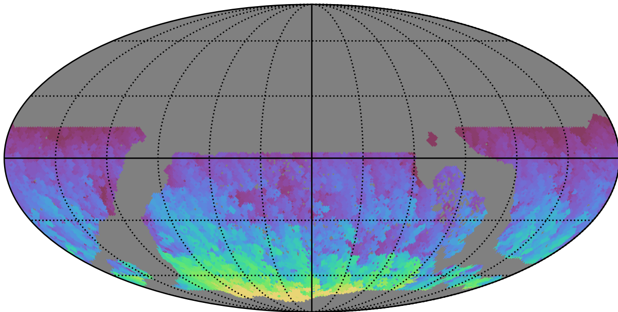
early_u_fpextra4.0_v3.4_10yrs WFD y band: Max HA
