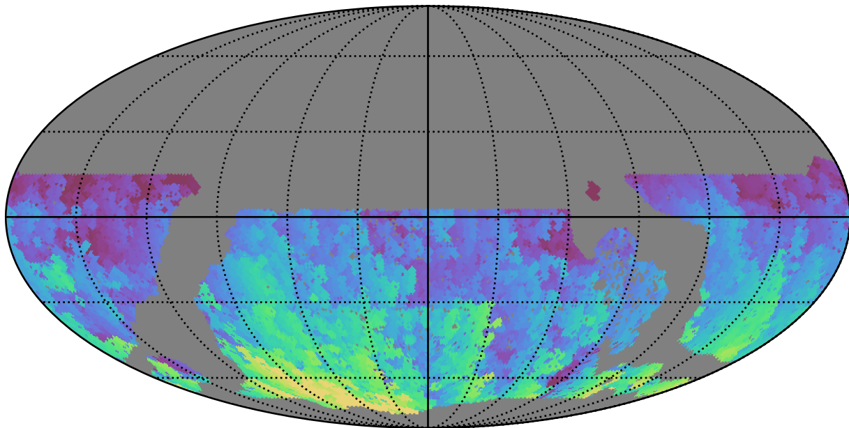
early_u_fpextra4.0_v3.4_10yrs WFD u band: Max HA
