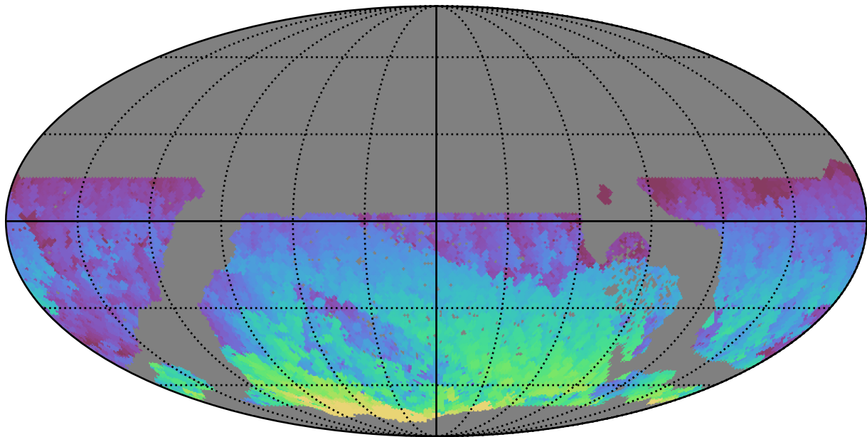
early_u_fpextra4.0_v3.4_10yrs WFD i band: Max HA
