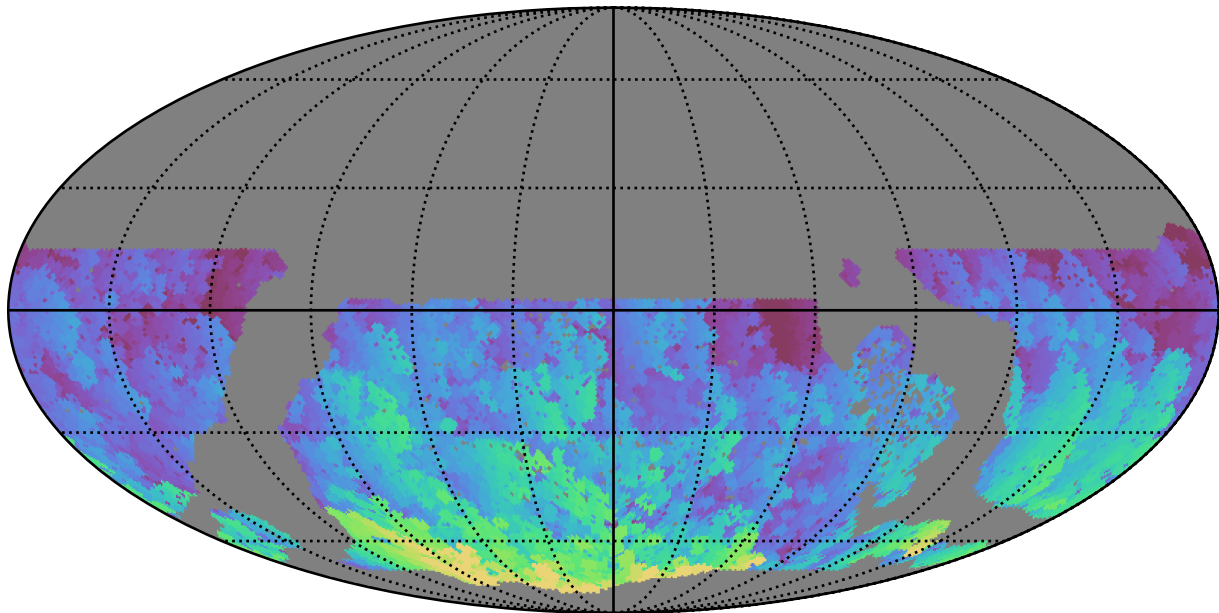
early_u_fpextra4.0_v3.4_10yrs WFD g band: Max HA
