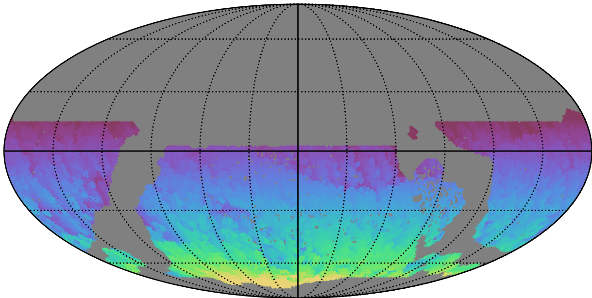
early_u_fpextra4.0_v3.4_10yrs WFD all bands: Max HA
