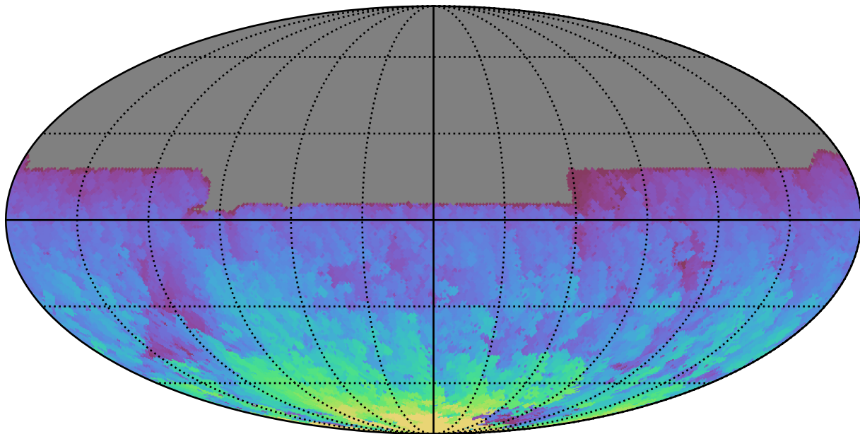
early_u_fpextra4.0_v3.4_10yrs All sky y band: Max HA
