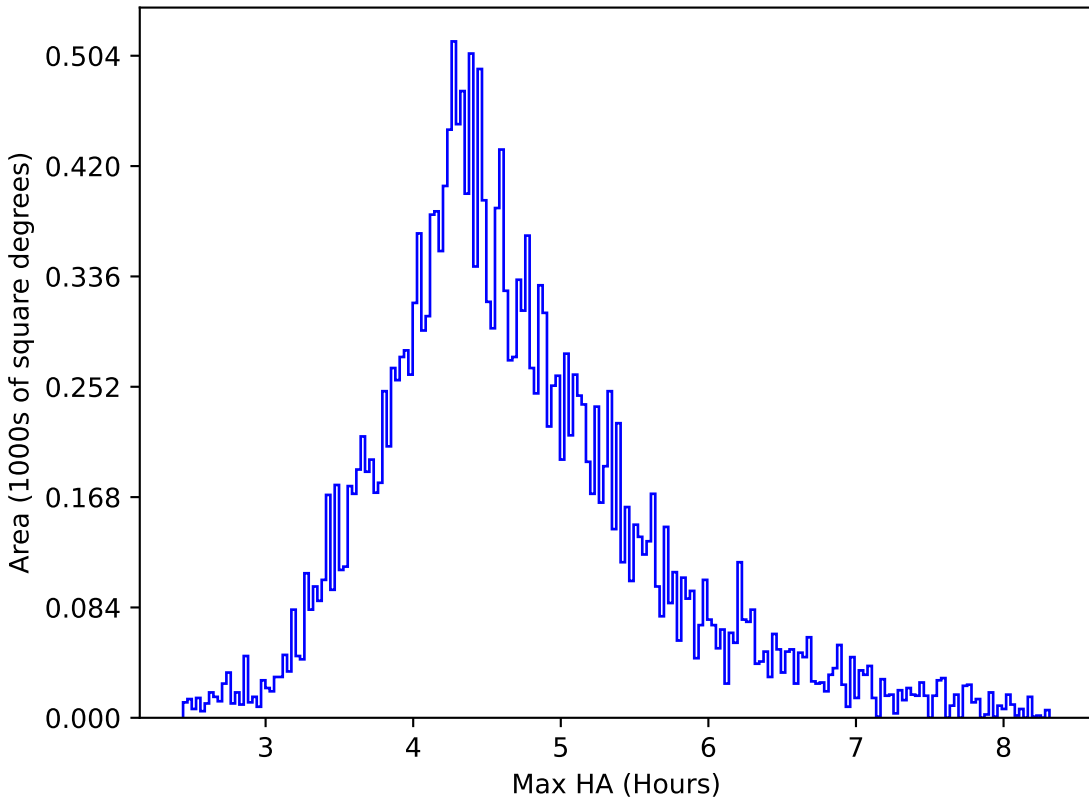
early_u_fpextra4.0_v3.4_10yrs All sky y band: Max HA
