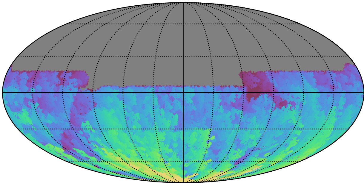
early_u_fpextra4.0_v3.4_10yrs All sky u band: Max HA
