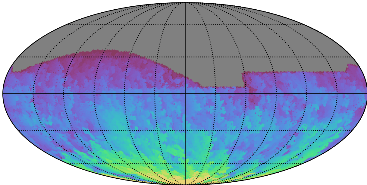
early_u_fpextra4.0_v3.4_10yrs All sky r band: Max HA
