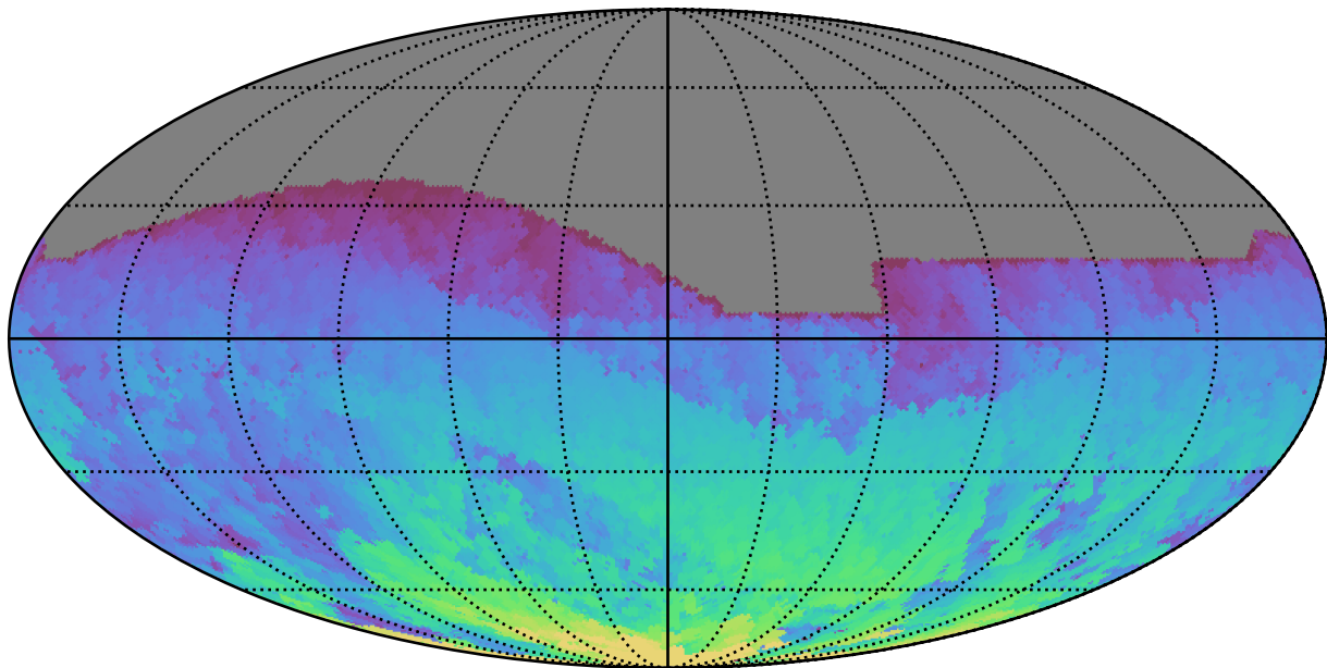
early_u_fpextra4.0_v3.4_10yrs All sky i band: Max HA
