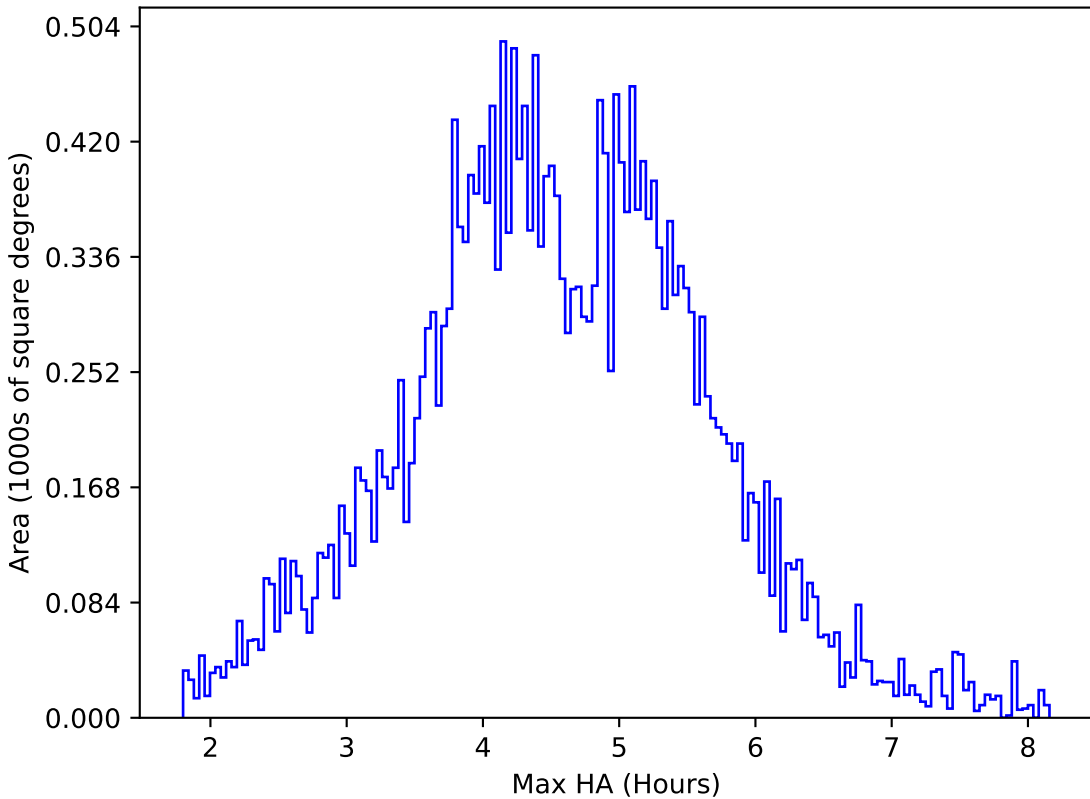
early_u_fpextra4.0_v3.4_10yrs All sky i band: Max HA
