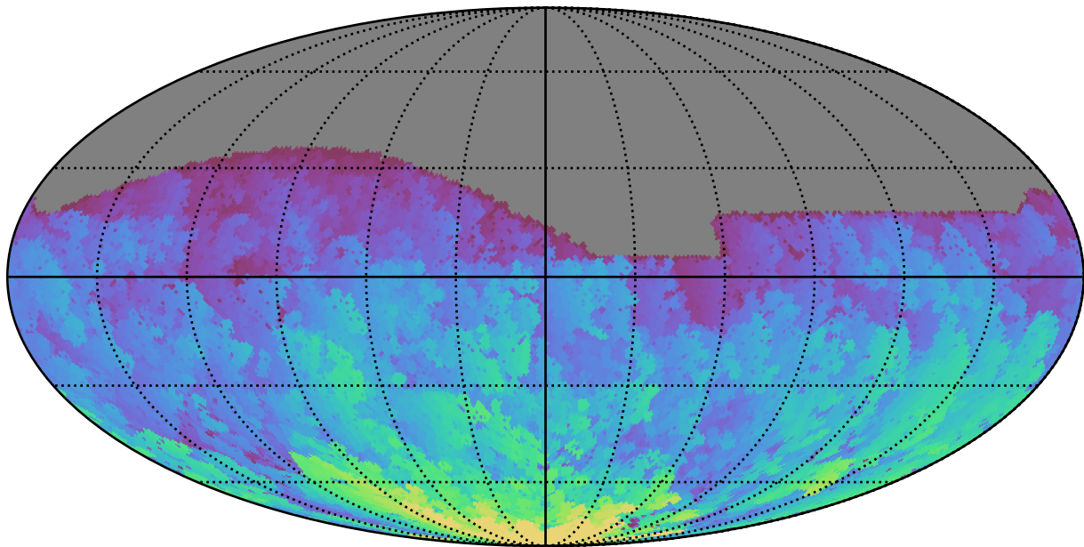
early_u_fpextra4.0_v3.4_10yrs All sky g band: Max HA
