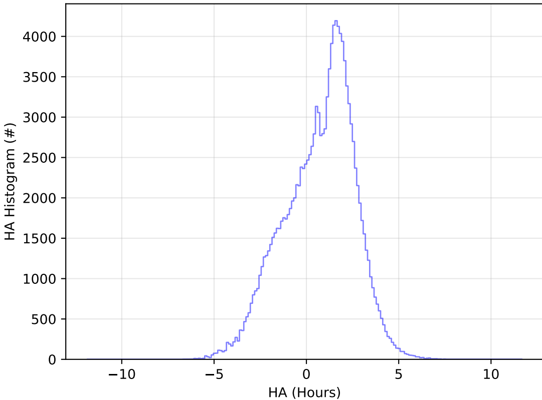
early_u_fpextra4.0_v3.4_10yrs WFD u band: HA Histogram
