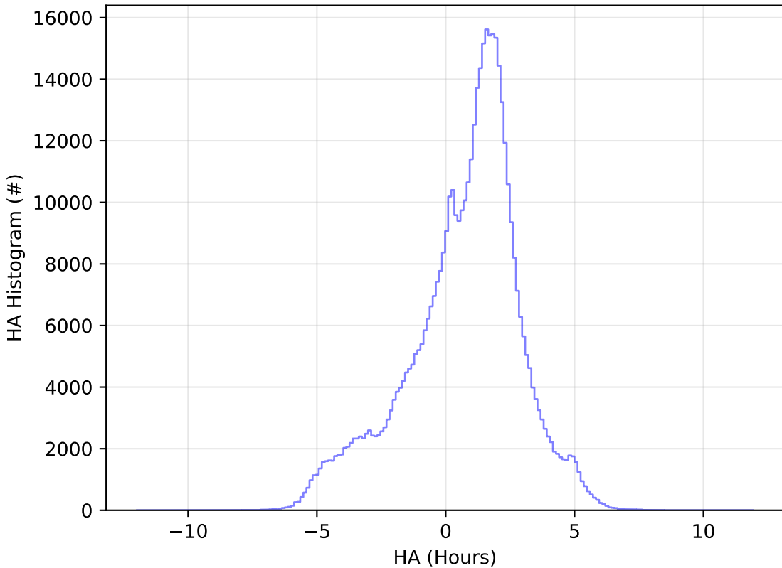
early_u_fpextra4.0_v3.4_10yrs WFD i band: HA Histogram
