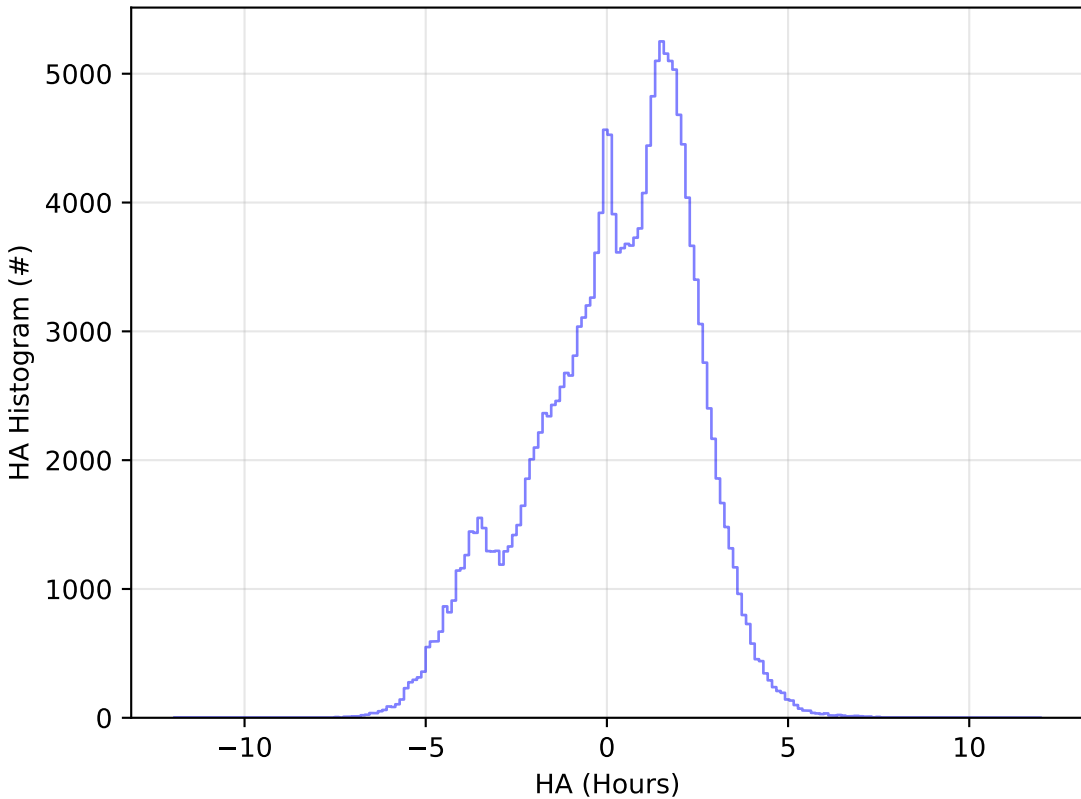
early_u_fpextra4.0_v3.4_10yrs WFD g band: HA Histogram
