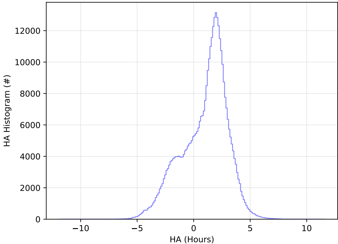
early_u_fpextra4.0_v3.4_10yrs All sky y band: HA Histogram
