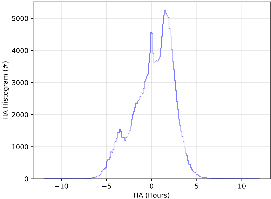
early_u_fpextra4.0_v3.4_10yrs All sky g band: HA Histogram
