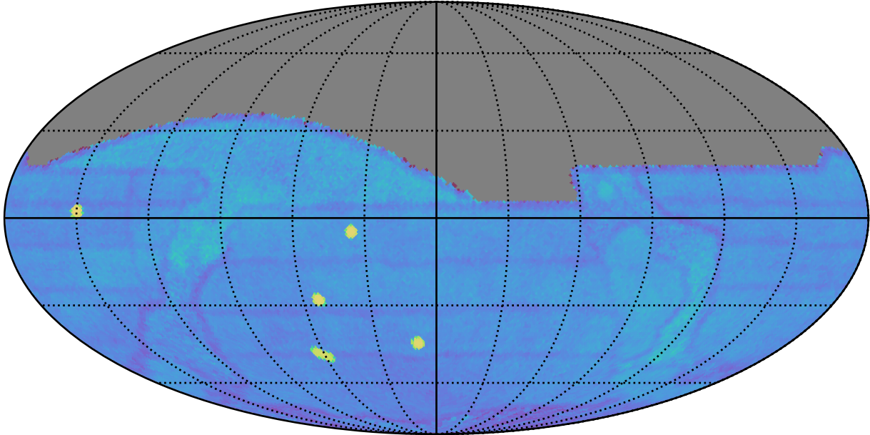
early_u_fpextra4.0_v3.4_10yrs gri All sky: Fraction of visits with a revisit < 60 min
