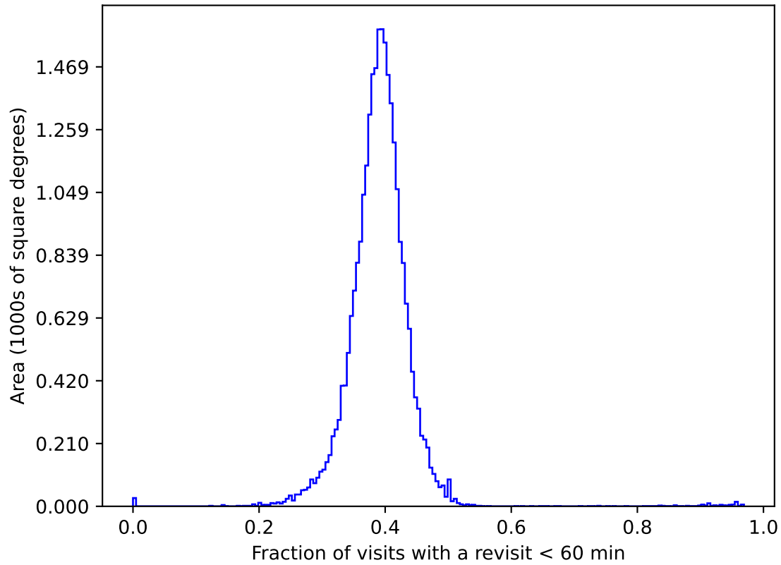
early_u_fpextra4.0_v3.4_10yrs gri All sky: Fraction of visits with a revisit < 60 min
