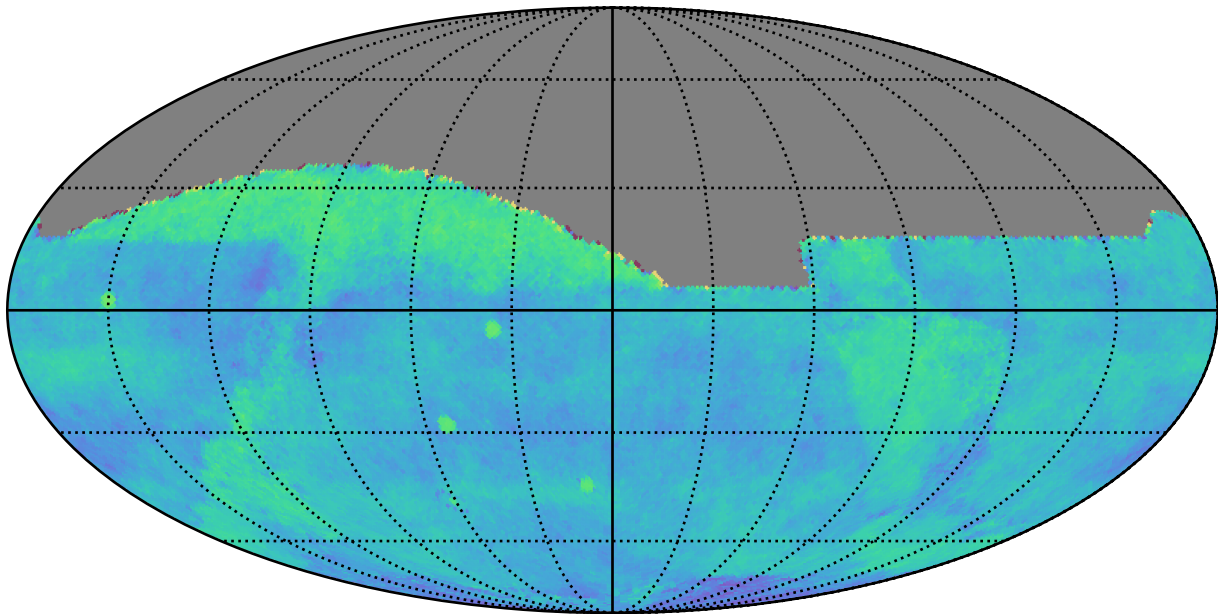
early_u_fpextra4.0_v3.4_10yrs gri All sky: Fraction of visits in pairs (20-90 min)
