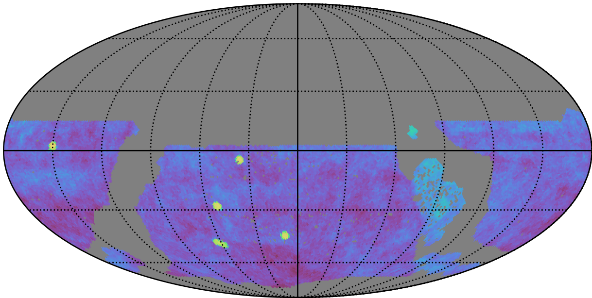
early_u_fpextra4.0_v3.4_10yrs gri WFD: Fraction of visits in pairs (10-60 min)
