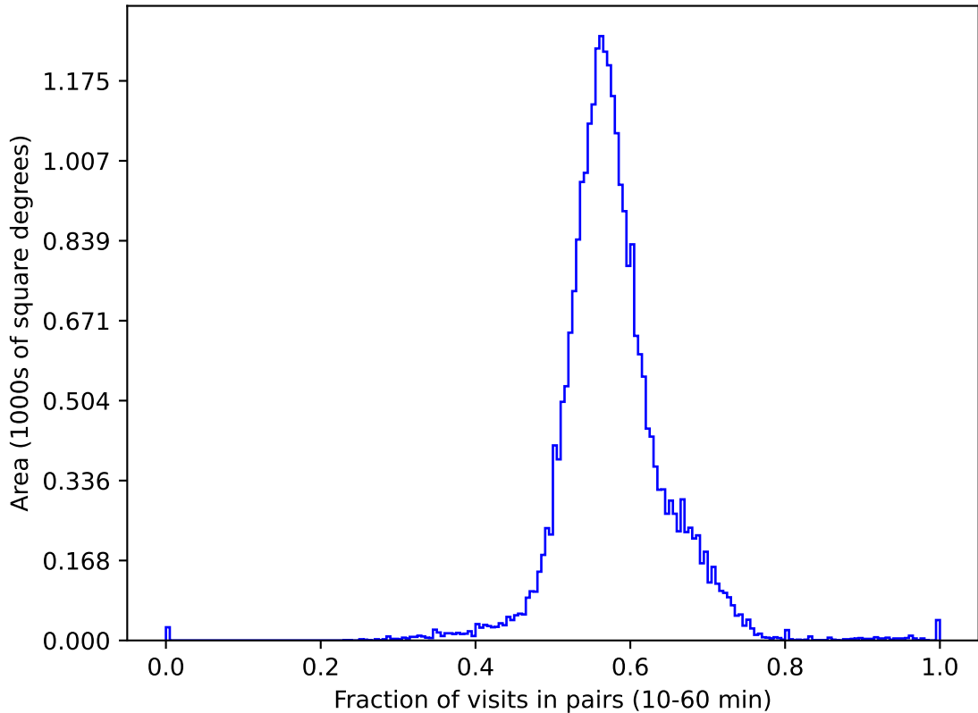
early_u_fpextra4.0_v3.4_10yrs gri All sky: Fraction of visits in pairs (10-60 min)
