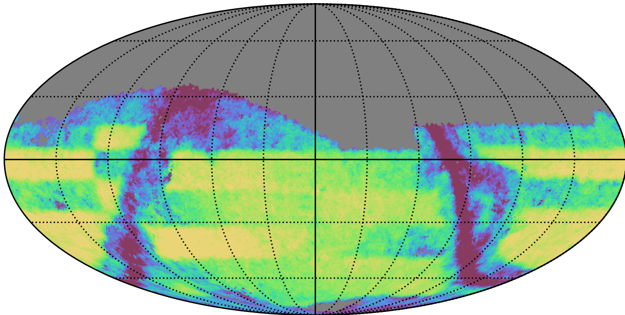
early_u_fpextra4.0_v3.4_10yrs Yr 3-4 z band: Exgal_CoaddM5
