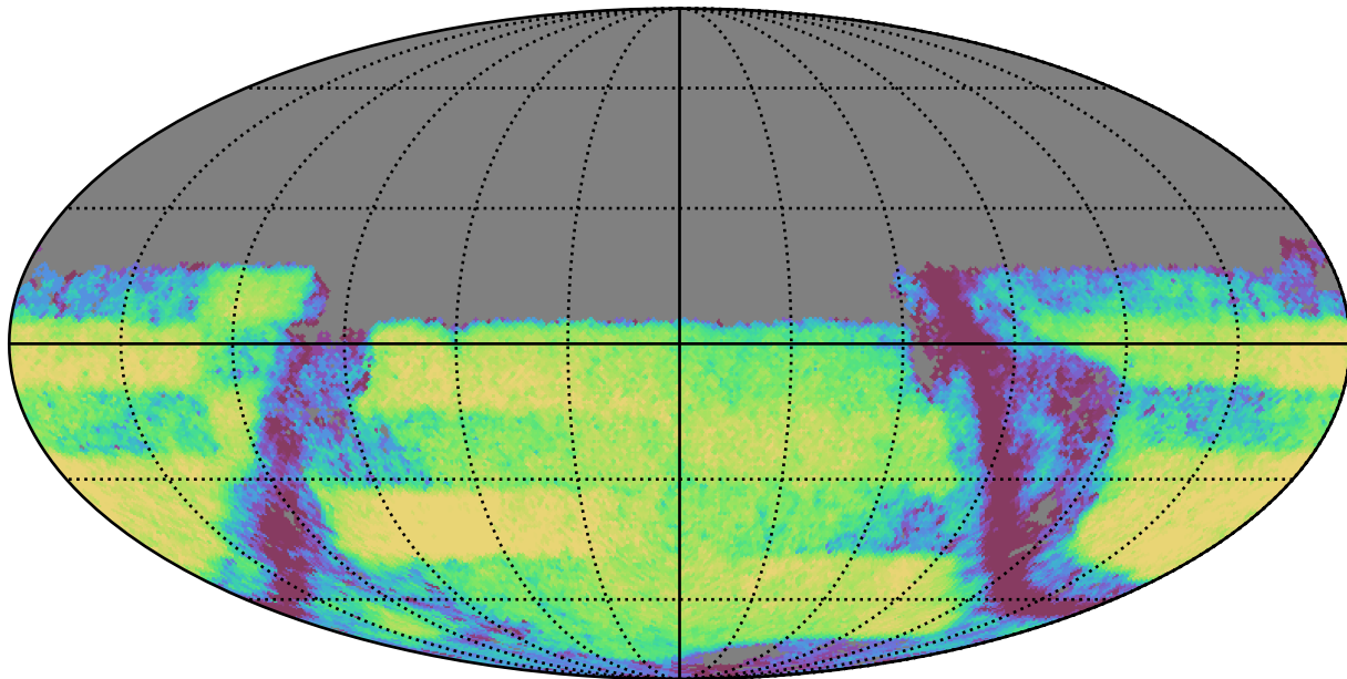
early_u_fpextra4.0_v3.4_10yrs Yr 3-4 y band: Exgal_CoaddM5
