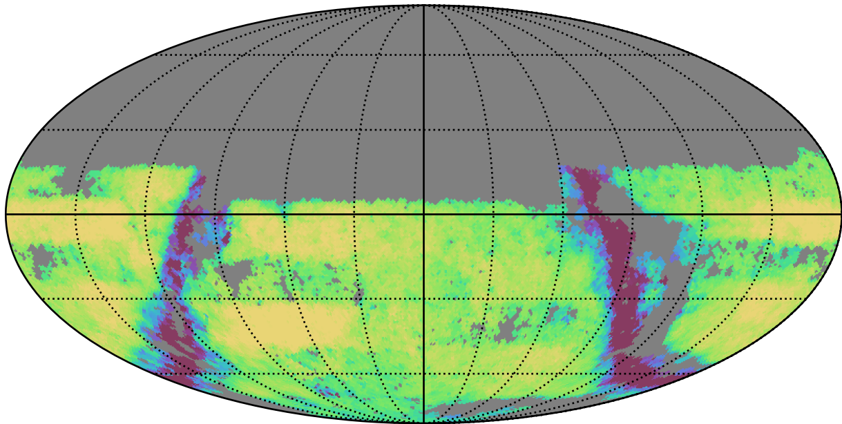
early_u_fpextra4.0_v3.4_10yrs Yr 3-4 u band: Exgal_CoaddM5
