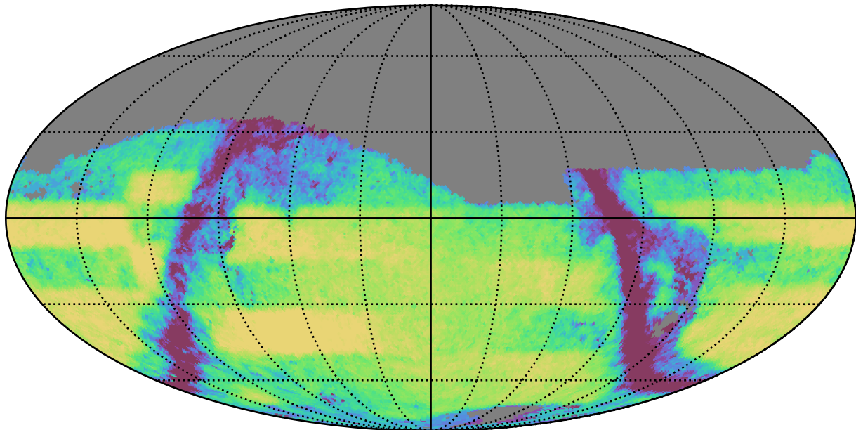
early_u_fpextra4.0_v3.4_10yrs Yr 3-4 r band: Exgal_CoaddM5
