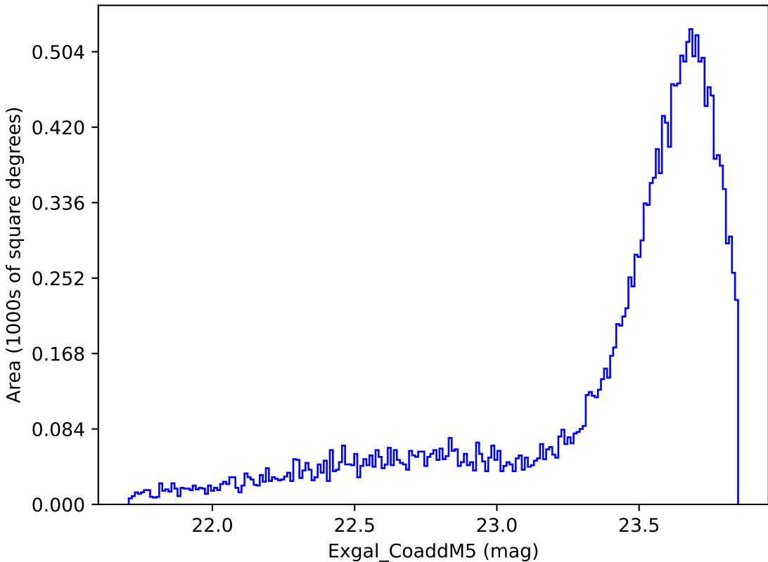
early_u_fpextra4.0_v3.4_10yrs Yr 1 y band: Exgal_CoaddM5
