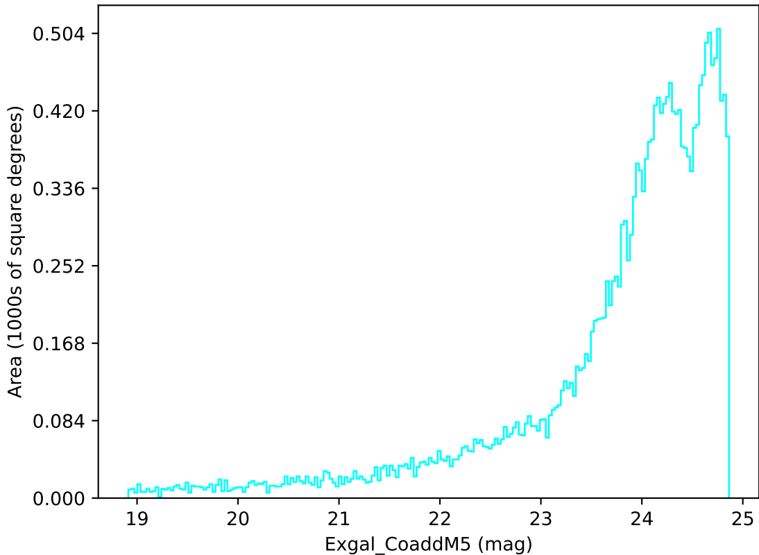
early_u_fpextra4.0_v3.4_10yrs Yr 1 u band: Exgal_CoaddM5
