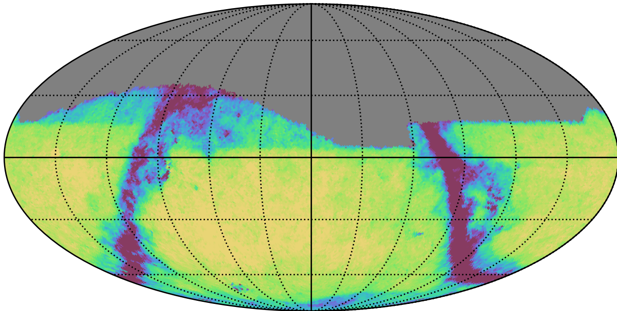
early_u_fpextra4.0_v3.4_10yrs Yr 1 r band: Exgal_CoaddM5
