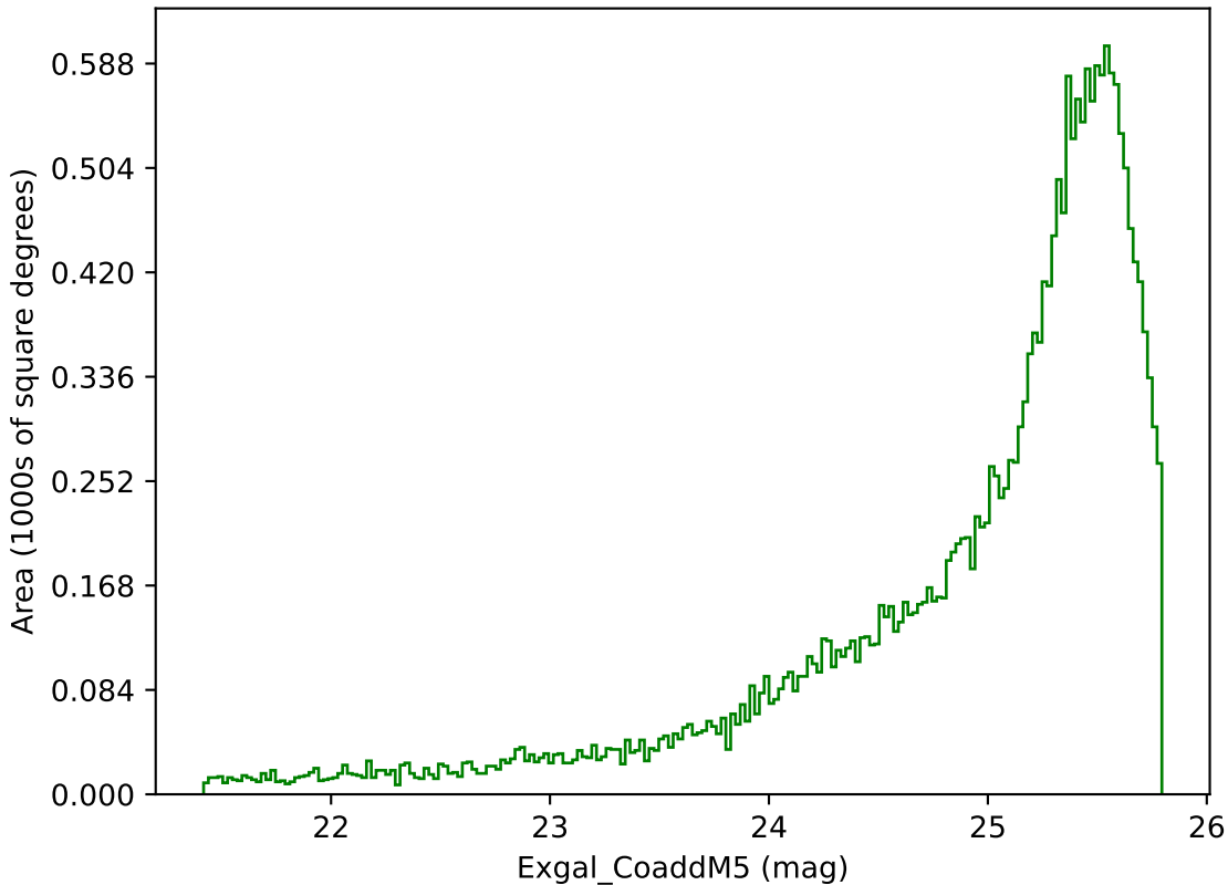
early_u_fpextra4.0_v3.4_10yrs Yr 1 g band: Exgal_CoaddM5
