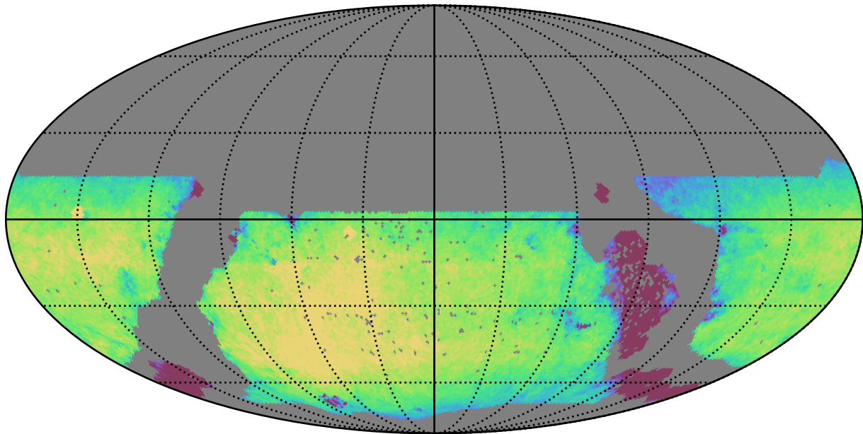
early_u_fpextra4.0_v3.4_10yrs WFD z band: Exgal_CoaddM5
