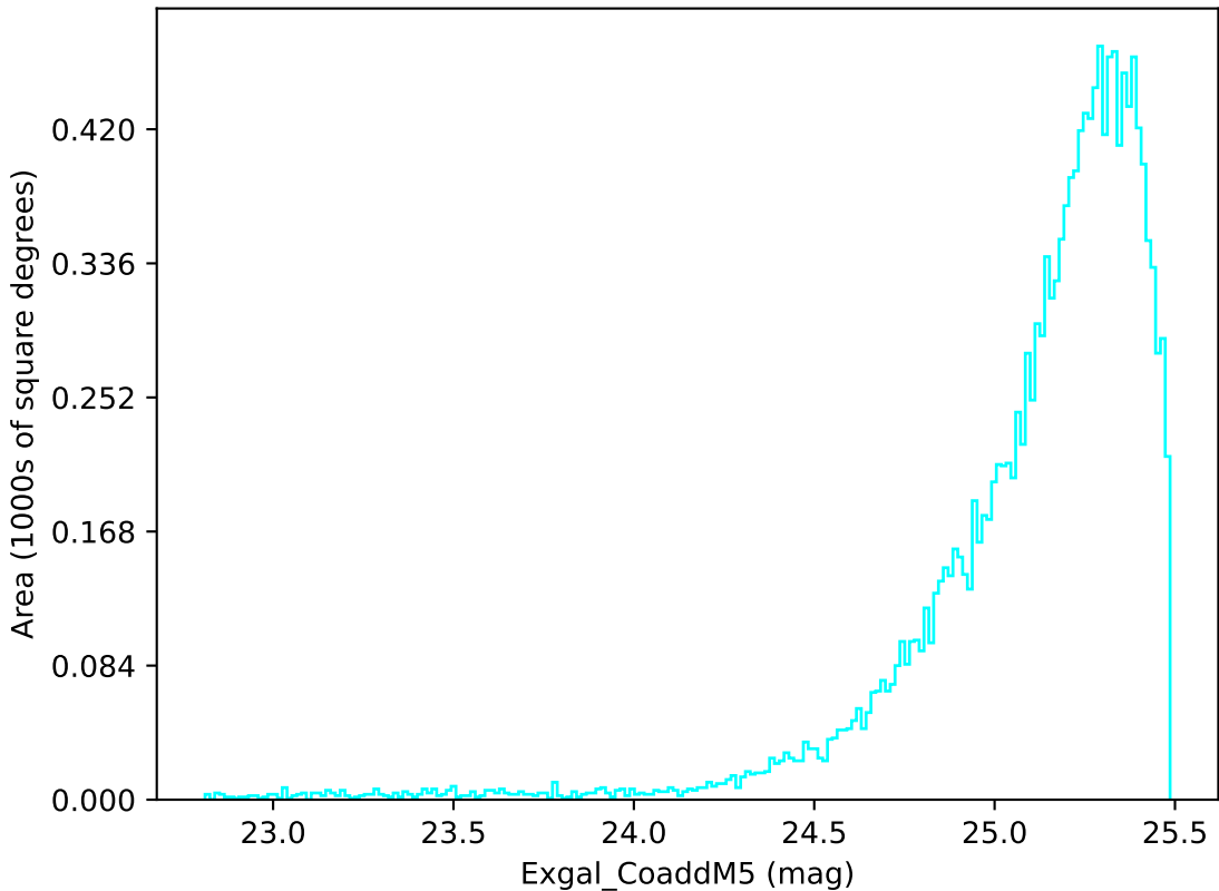
early_u_fpextra4.0_v3.4_10yrs WFD u band: Exgal_CoaddM5
