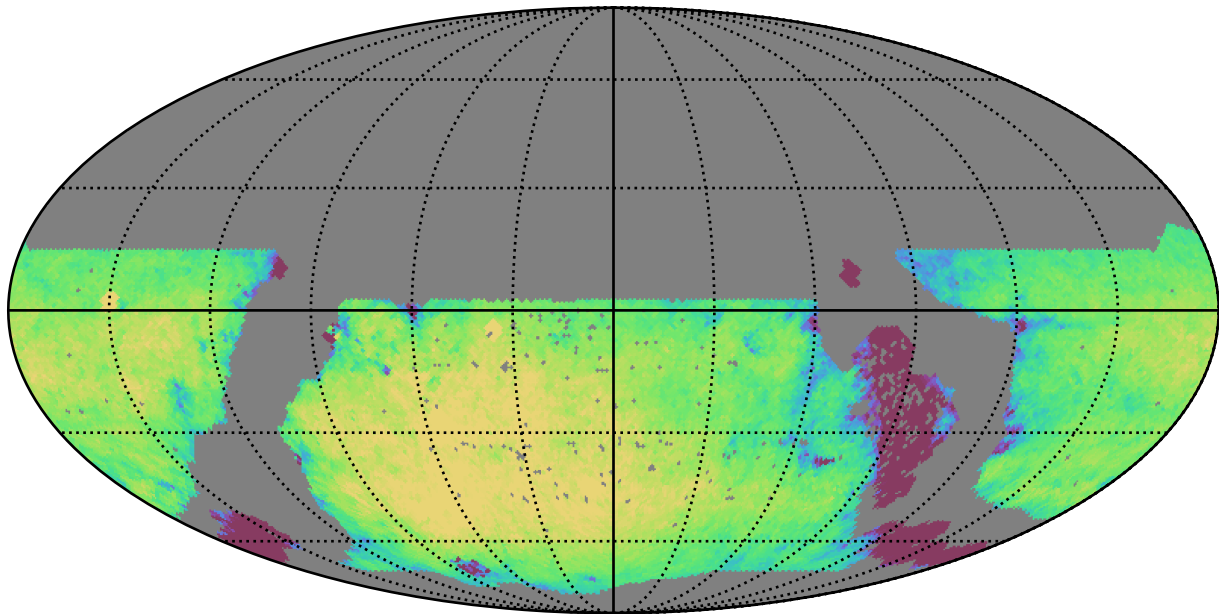
early_u_fpextra4.0_v3.4_10yrs WFD g band: Exgal_CoaddM5
